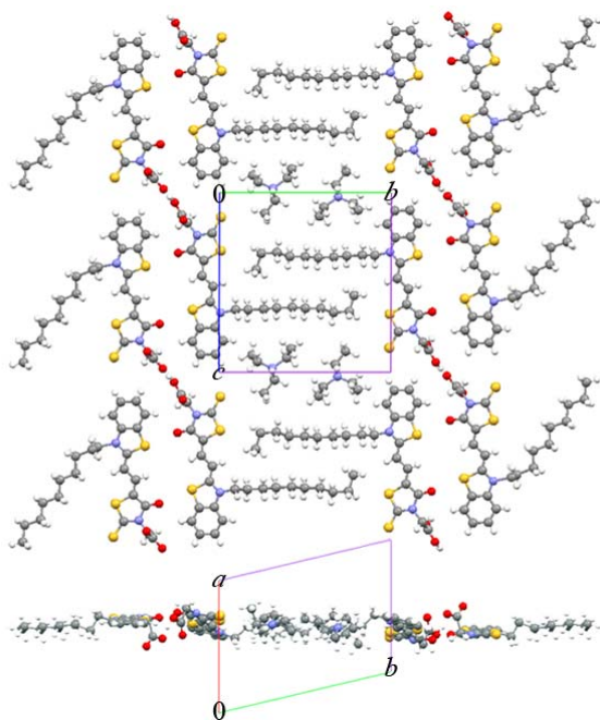
Fig. 4S Packing structure of merocyanine dye's salt viewed down the a axis (Top) and the c axis (Side).
